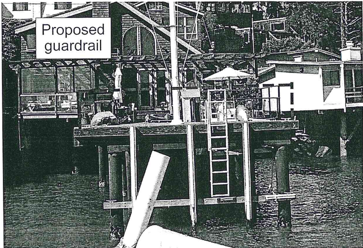
Figure 2: Existing pier, viewed from the south
